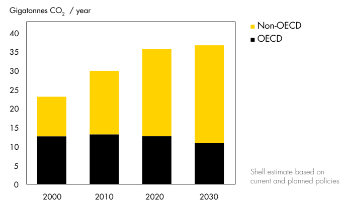
Chart 6. CO 2 Pathways
