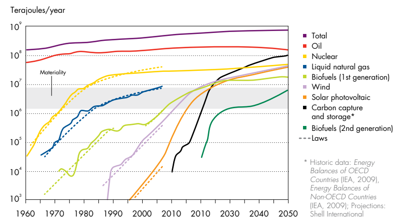
Chart 8. Energy-Technology Deployment
